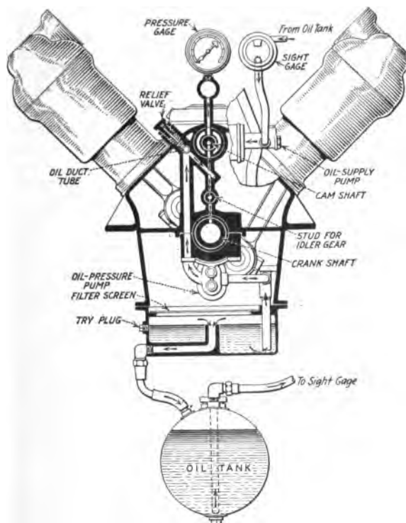
FIG. 78.—Oiling system.
