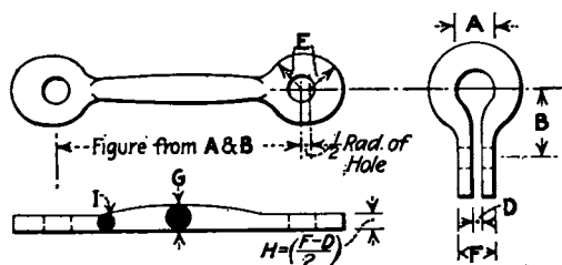
FIG. 50.—Shackles.
