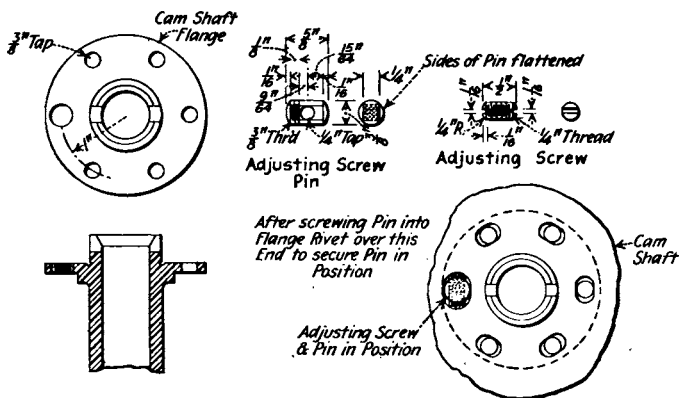
FIG. 74.—Lining up camshaft gear.
