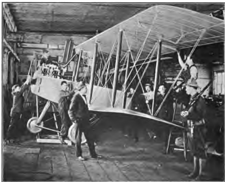
FIG. 122.—Front of training machine.
