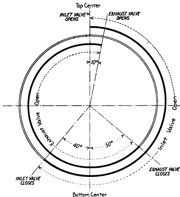
FIG. 85.—Timing diagram.
