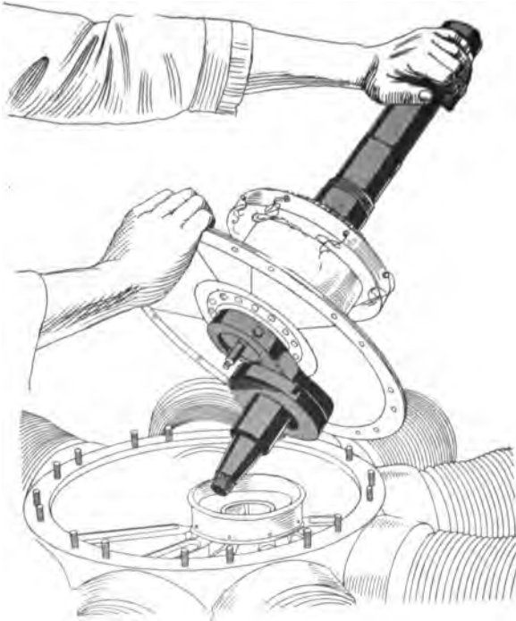
FIG. 100.—Assembling crankshaft.
